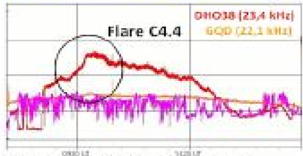
Double-Spot flare left & SID above on 14 Aug
