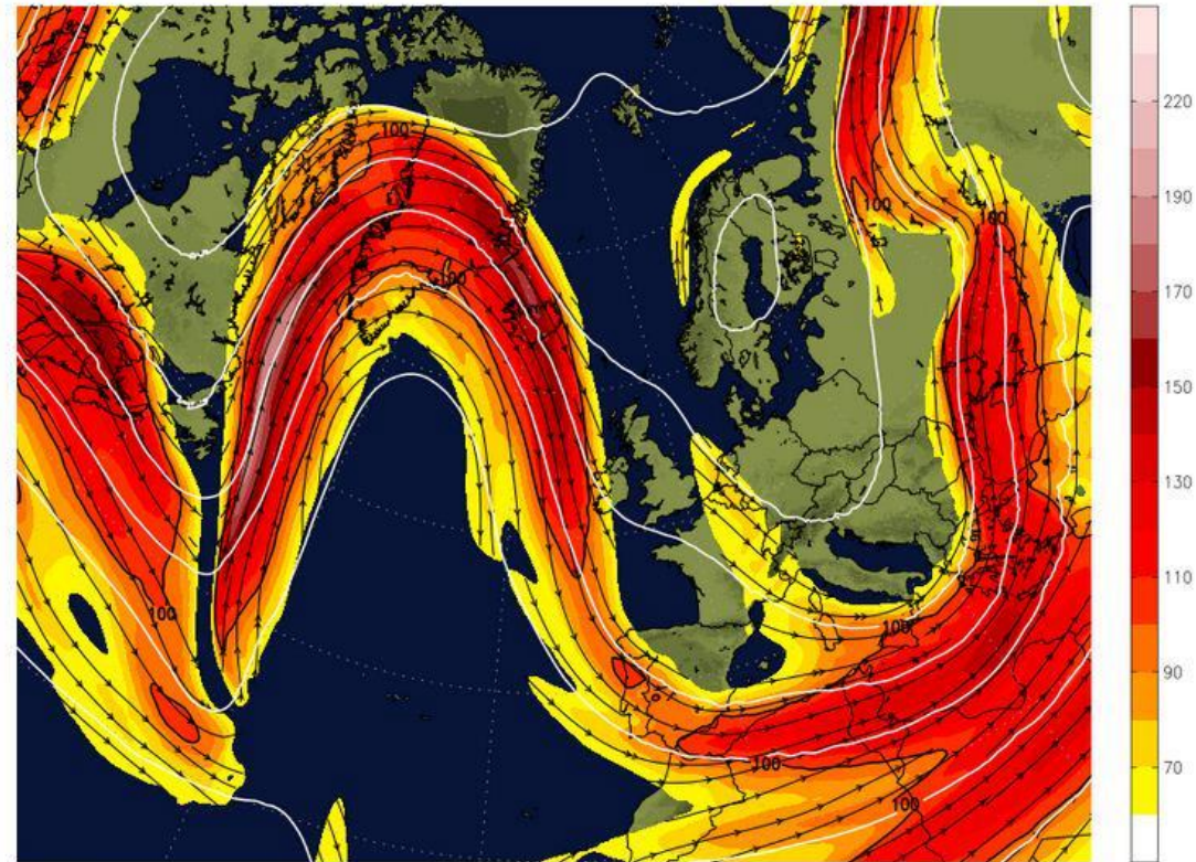
(Above) Jet Stream – ‘displaced Polar Vortex’ – 2 Feb confirming WeatherAction 6 months ahead (extract below)
