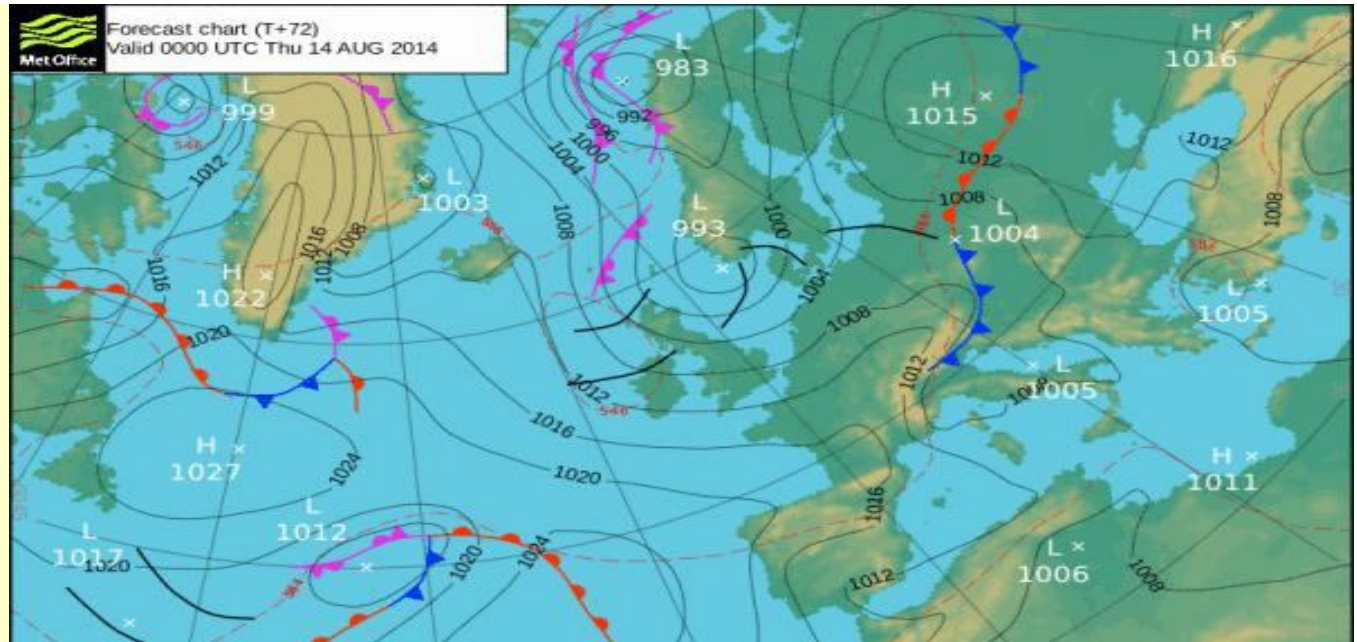
WEATHERACTION 2014 AUGUST (3-30d) ahead fc Europe detail SLAT10 produced 30 th July from choices made mid-July. General reportage welcome but any publication of details in media or web must be agreed through www.weatheraction.com Confidential. © Weather Action (+44/0)2079399946
