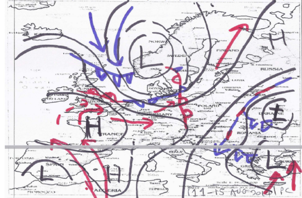
Europe Possible Pressure Scenario Map SLAT 10 AUGUST 2014 for: 11 th – 15 th August Confidence: B = 75% Prod 30 th July from choices made mid-July. Timing to 1 day. Likely success rate of weather periods is 8 or 9 basically successful out of every 10
