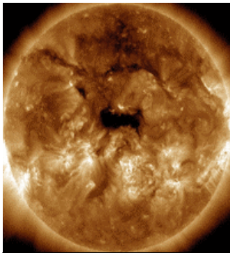
Earth-Facing Coronal Hole ~4Dec, WeatherAction forecast map for STORM winds prod 14 Nov (Rt) WeatherAction forecast poss Press and MetO 0z5Dec OBS (far Rt)
