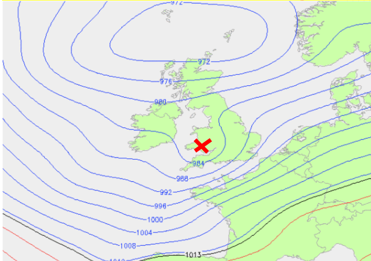
Surface Pressure GFS (hPa)
