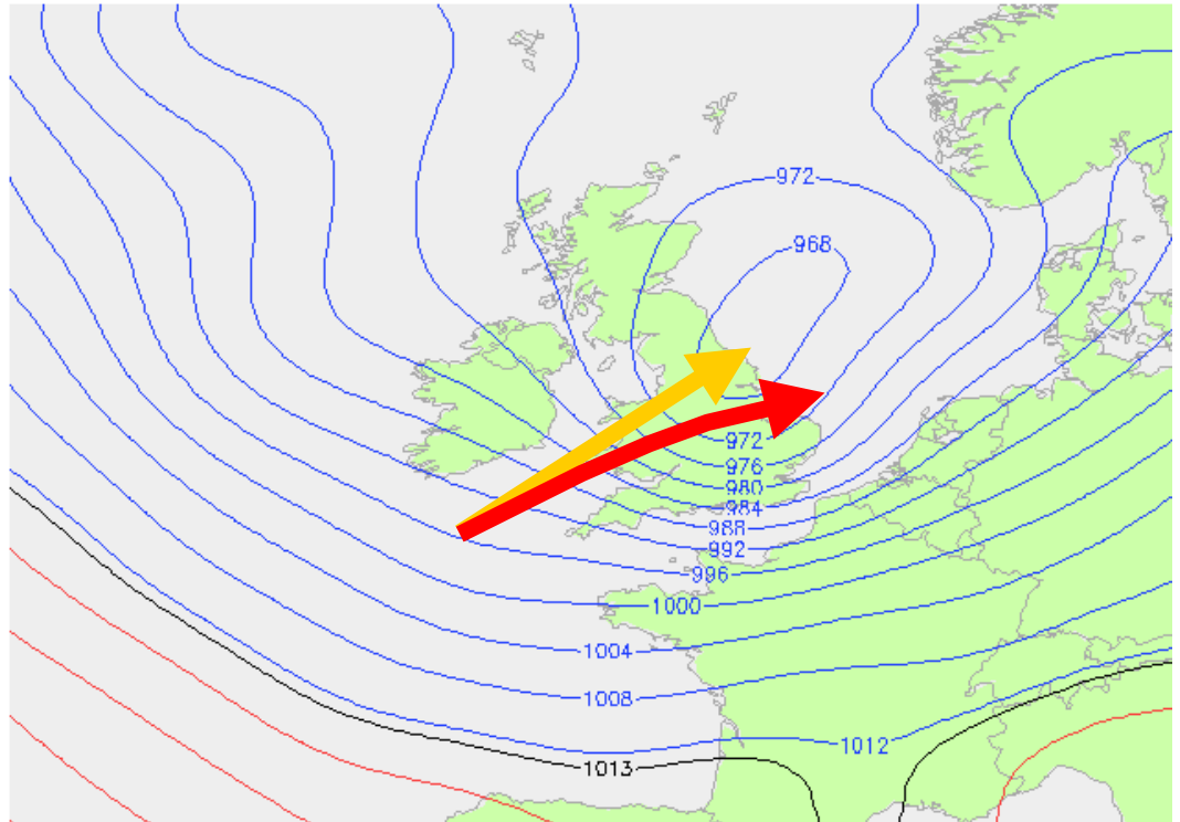
Surface Pressure GFS (hPa)
