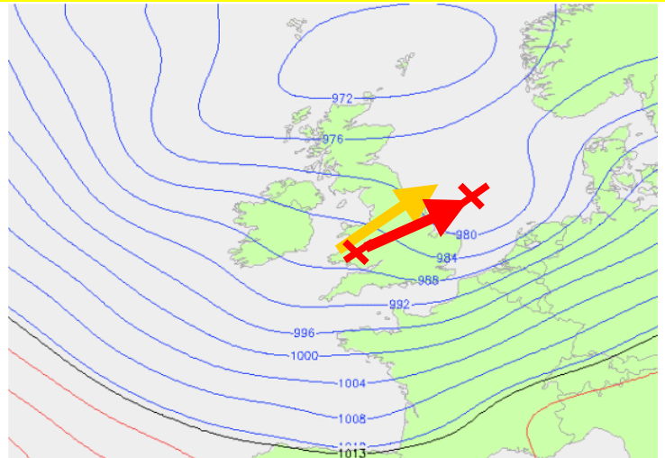
Surface Pressure GFS (hPa)
