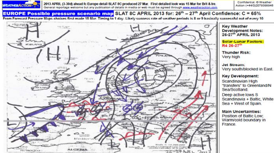
reas Map SLAT 8C APRIL 2013 for: 26 th – 27 th April es first made 15 Mar. Timing to 1 day. Likely success rate of weather pe
