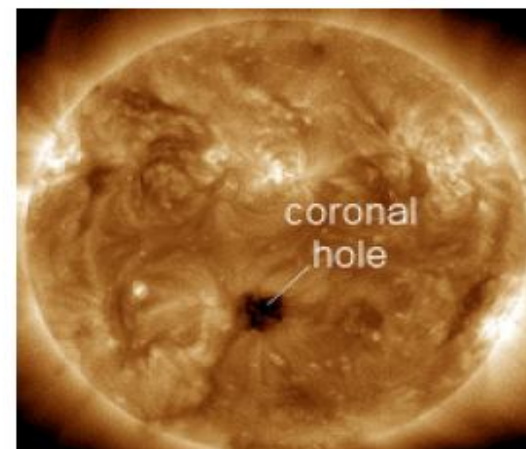
Example of Solar Action driving weather. Coronal Hole Jan9 http://bit.ly/YM7s6L implied (SLAT) main solar-Earth effect Jan10 - 13/14
