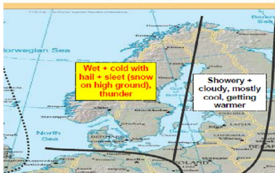
reas Map SLAT 8C APRIL 2013 for: 26 th – 27 th April es first made 15 Mar. Timing to 1 day. Likely success rate of weather pe
