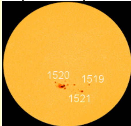
Sunspot 1520 has a delta-class magnetic field that harbors energy for X-class solar flares. Credit: SDO/HMI
