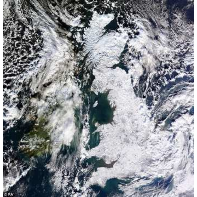
Snow covered Britain & Ireland from Space (NASA photo 7th Jan 2010) confirming WeatherAction Long range forecast issued July 2008, ahead of all others.
